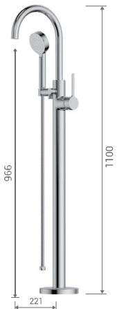
HWY0611-D01CP Freestanding bathtub mixer filler Brass body, 40mm cartridge, chrome.
