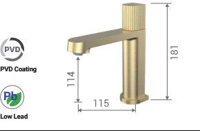
HWM0201-A01BV Basin mixer Brass body, energy saving cartridge, brushed bronze.
