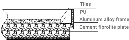
Connect method between waterproof plate and wall panel
