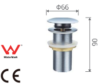
HDGD0037 Basin drainer G1 1/4", pop-up type, brass body, chrome.
