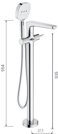
HWY0901-D01CP Freestanding bathtub mixer filler Brass body, 40mm cartridge, chrome.
