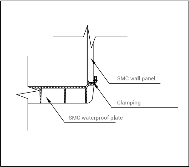
Connect method between waterproof plate and wall panel
