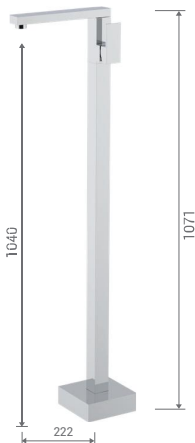
HWY5014-D01CP Freestanding bathtub mixer filler Brass body, 40mm cartridge, chrome.
