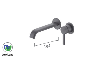
HWM0102-R01GD Wall mounted basin mixer Brass body, 35mm cartridge, gun grey.
