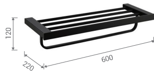
HDC8720-BK Bath towel shelf SUS304, matte black.
