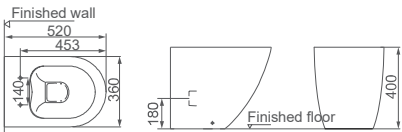
HDC877BTW Aqua Vortex Washdown Floorstanding Toilet Back To Wall Size 520x360x400mm P-trap P=180mm roughing-in 3/4.5L
