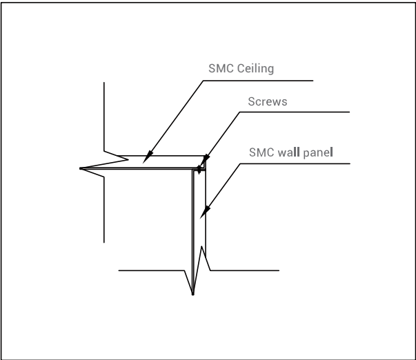
Connect method between ceiling and wall panels
