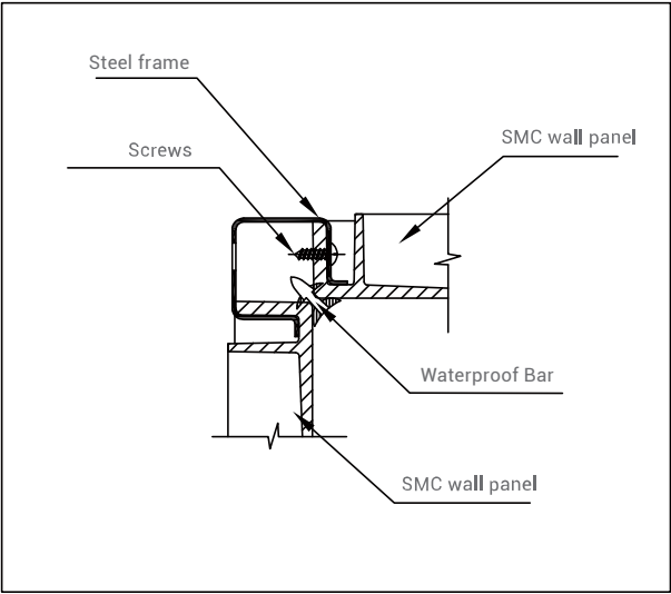
Connect method between wall panels(Corner)
