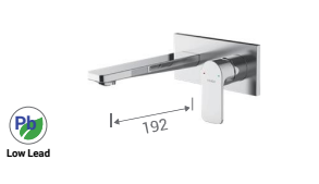
HWM0801-R09CP Wall mounted basin mixer Brass body, 35mm cartridge, chrome,
