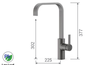
HWX0102-P01GD Kitchen sink mixer Brass body, 35mm cartridge, gun grey.
