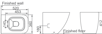
HDC879BTW Aqua Vortex Washdown Floorstanding Toilet Back To Wall Size 520x360x412mm P-trap P=180mm roughing-in 4/6L
