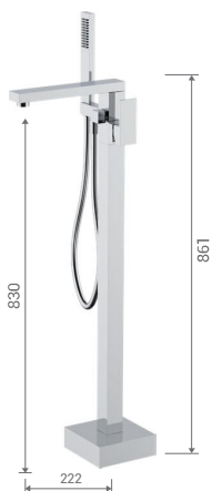
HWY5017-D01CP Freestanding bathtub mixer filler Brass body, 40mm cartridge, chrome.
