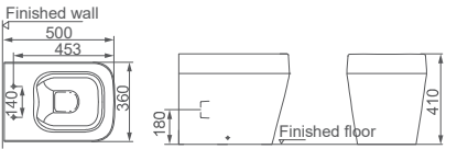
HDC540RBTW Rimless Washdown Floorstanding Toilet Back To Wall Size 500x360x410mm P-trap P=180mm roughing-in 4/6L
