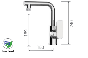
HWM0801-A05CP Basin mixer Brass body, multi-function spout, 35mm cartridge, chrome,
